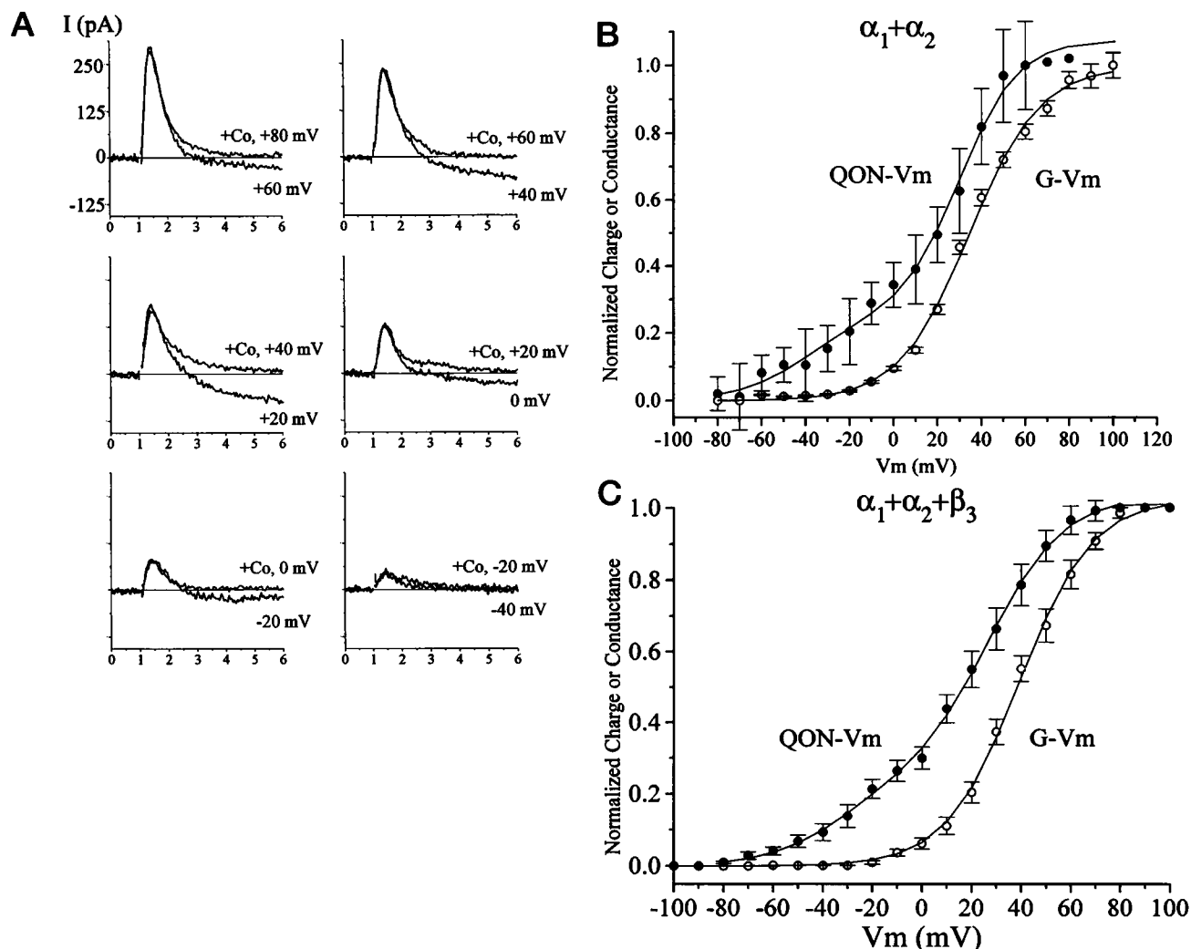
FIGURE 8 A comparison of the voltage dependence for the activation of the human L-type cardiac \text{Ca}^{2+} channel charge movement and conductance. (A) The method used to determine the amount of surface charge shift produced by the addition of 5 mM \text{Co}^{2+} in the charge movement experiments. Examples are shown of the superimposition of a family of gating currents recorded at +80, +60, +40, +20, 0, and -20 mV (after \text{Co}^{2+} , labeled +Co, upper traces) with the gating current plus calcium current traces in the same cell ( I_g and I_{Ca} ) at +60, +40, +20, 0, -20, and -40 mV (before \text{Co}^{2+} , lower traces); current and time calibrations: 125 pA/div, 1.0 ms/div. (B and C) The voltage dependence for the Ca channel charge movement ( \bullet ) and for the Ca channel conductance ( \circ ) with the \alpha_1 + \alpha_2 (B) and with the \alpha_1 + \alpha_2 + \beta_3 subunits (C). The G-Vm curve was shifted by +20 mV on the voltage axis to offset the surface charge shift produced by the 5 mM \text{Co}^{2+} used in the charge movement experiments. The calcium channel conductance was measured using a tail current method, after the subtraction of the OFF gating currents. The Boltzmann fits (solid lines) were calculated using the data from -80 to +80 mV and were drawn using the following parameters: for A: G-Vm: G_{\max} , 1.0 (0.1); V , 34.5 (0.7) mV; K , 15.8 (0.6) mV; and for QON-Vm: Q_{\max 1} , 0.25 (0.2); V_1 , -38.8 (12.5) mV; K_1 , 15.9 (3.5) mV; and Q_{\max 2} , 0.81 (0.1); V_2 , 29.9 (1.1) mV; K_2 , 13.1 (1.8) mV; for B: G-Vm: G_{\max} , 1.0 (0.1); V , 39.1 (0.5) mV; K , 14.5 (0.4) mV; and for QON-Vm: Q_{\max 1} , 0.24 (0.1); V_1 , -32.1 (12.2) mV; K_1 , 15.7 (4.5) mV; and Q_{\max 2} , 0.79 (0.1); V_2 , 26.9 (3.3) mV; K_2 , 15.1 (2.2) mV.
