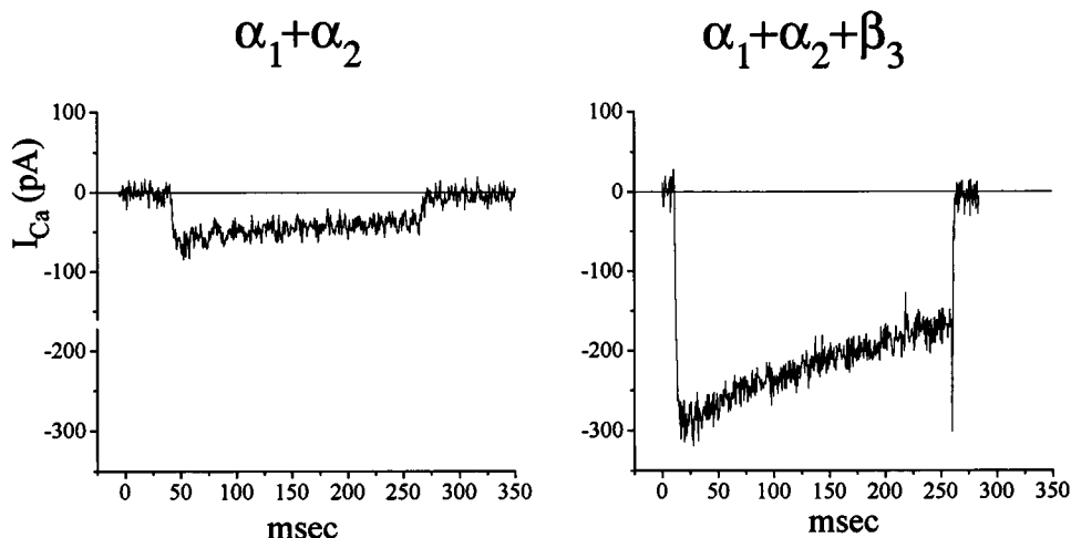
FIGURE 1 Calcium channel (ionic) currents recorded from HEK293 cells transfected with human cardiac L-type Ca channel subunits. ( Left ) (labeled \alpha_1 + \alpha_2 ) A \text{Ca}^{2+} current recorded after transfection with human \alpha_1 and rabbit \alpha_2 subunits. ( Right ) (labeled \alpha_1 + \alpha_2 + \beta_3 ) A \text{Ca}^{2+} current recorded after transfection with human \alpha_1 , rabbit \alpha_2 , and human \beta_3 subunits. Both currents were recorded from a holding potential of -100 mV, to a test voltage of +20 mV. The external solution contained 1.8 mM \text{Ca}^{2+} ions. The cell input capacitance was 22 pF and 24 pF for ( \alpha_1 + \alpha_2 ) and ( \alpha_1 + \alpha_2 + \beta_3 ).
