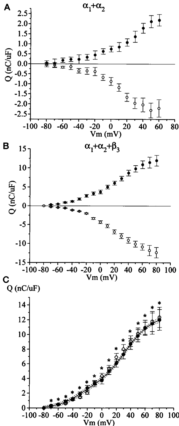
FIGURE 6 The QON- V_m and QOFF- V_m curves for the human cardiac L-type \text{Ca}^{2+} channels composed of \alpha_1 + \alpha_2 subunits (A, n = 7 ) and for the \alpha_1 + \alpha_2 + \beta_3 subunits (B and C; n = 8 ). QON and QOFF were obtained by integration of the ON (●) and OFF (○) \text{Ca}^{2+} channel gating currents. C is a plot of QON (●) and the absolute value of QOFF (○) for direct comparison. The mean QON data were fit (solid line) by a sum of two Boltzmann expressions, with the following parameters: Q_{\text{max}1} , 2.74 (0.82) nC/ \mu\text{F} ; V_1 , -34.8 (6.4) mV; K_1 , 14.3 (2.9) mV; and Q_{\text{max}2} , 9.96 (1.1) nC/ \mu\text{F} ; V_2 , 32.6 (2.4) mV; K_2 , 18.4 (2.2) mV. Also plotted are the 99% confidence limits for the Boltzmann fit (dotted lines). The asterisks and stars above each set of symbols indicate the statistical probabilities that the QON and QOFF are different; asterisks indicate p < 0.05 , and stars indicate p < 0.005 . In A, B, and C the charge data from each cell were normalized to the cell input capacitance and then averaged to give values in units of nC/ \mu\text{F} . The data points are the means \pm SE.
