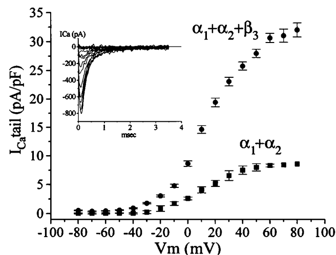
FIGURE 3 The voltage dependence for the conductance of human L-type cardiac \text{Ca}^{2+} channels composed of \alpha_1 + \alpha_2 subunits ( \blacksquare , n = 10 ), or \alpha_1 + \alpha_2 + \beta_3 subunits ( \bullet , n = 14 ). The conductance was estimated by measuring the peak tail currents after repolarization to -100 mV after 5.4 -ms test steps. The OFF gating current was subtracted from the peak tail current amplitude. The resulting absolute value of the ionic tail current amplitude was normalized to the cell input capacitance before averaging. The inset shows examples of the time course of the tail currents ( \alpha_1 + \alpha_2 + \beta_3 subunits) in response to voltage steps to -80 through +60 mV.
