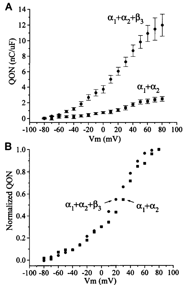
FIGURE 7 A comparison of the voltage dependence of QON for the \alpha_1 + \alpha_2 (■) and \alpha_1 + \alpha_2 + \beta_3 (●) subunit combinations. (A) Comparison of QON for the two subunit combinations. (B) Same data as shown in A, but each data set was normalized to its Q_{\text{max}} value.
