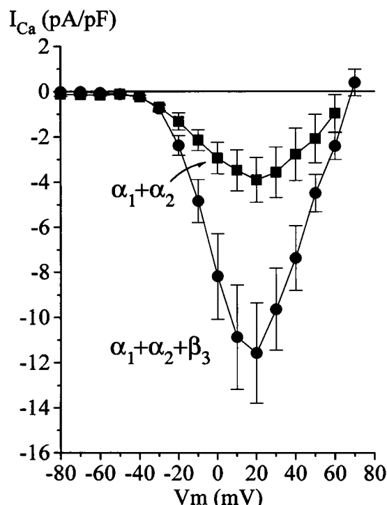
FIGURE 2 The current-voltage relationships for the peak inward L-type cardiac \text{Ca}^{2+} current density (pA/pF) recorded from HEK293 cells transfected with \alpha_1 + \alpha_2 subunits ( \blacksquare , n = 8 ), or \alpha_1 + \alpha_2 + \beta_3 subunits ( \bullet , n = 9 ). The mean \text{Ca}^{2+} current density \pm SD is given; the data from each cell were normalized by the cell input capacitance.
